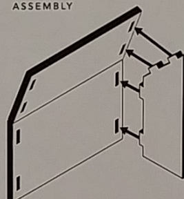
HAND GUARD RIGHT-HANDED ASSEMBLY
